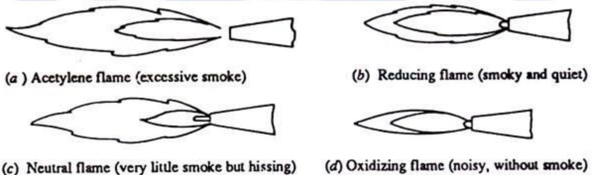
Fig. 16-15 Structures of different types of oxy-acetylene flames.
