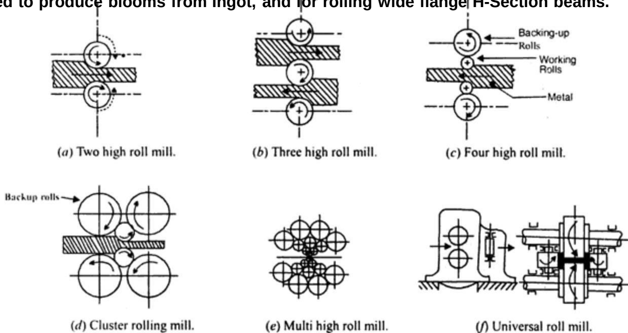
Fig. 2.9. Types of rolling mills.
