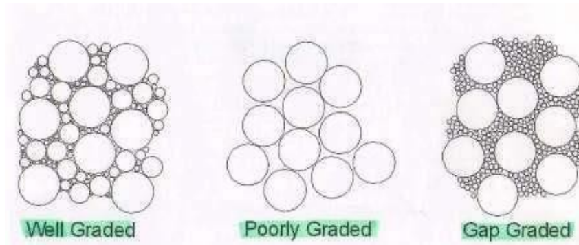
Fig.7: aggregate grading types
