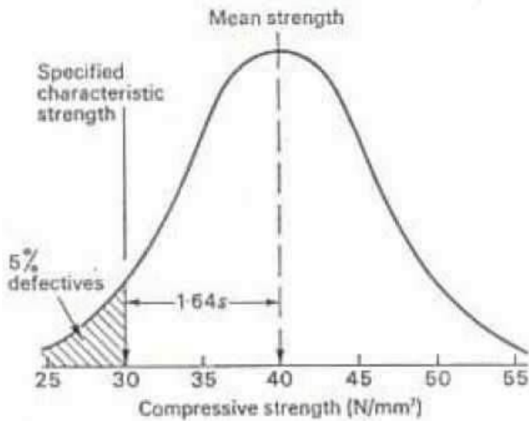
Fig.1: Means compressive strength vs characteristic compressive strength
